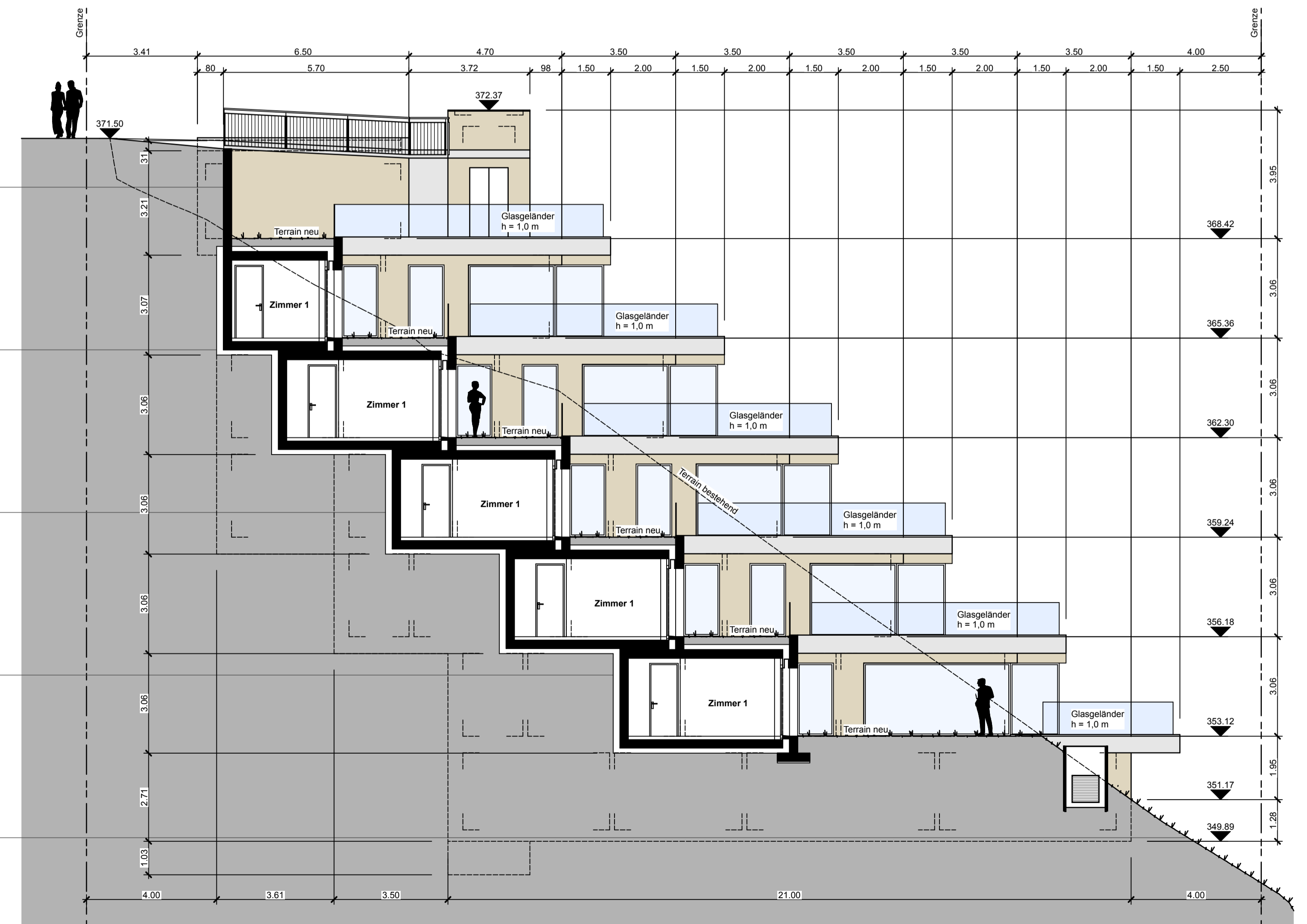
Nord-West Fassade
